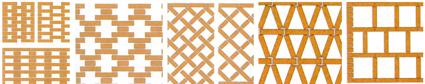
A CORSI SFALSATI/ IN ALTERNATED COURSES
